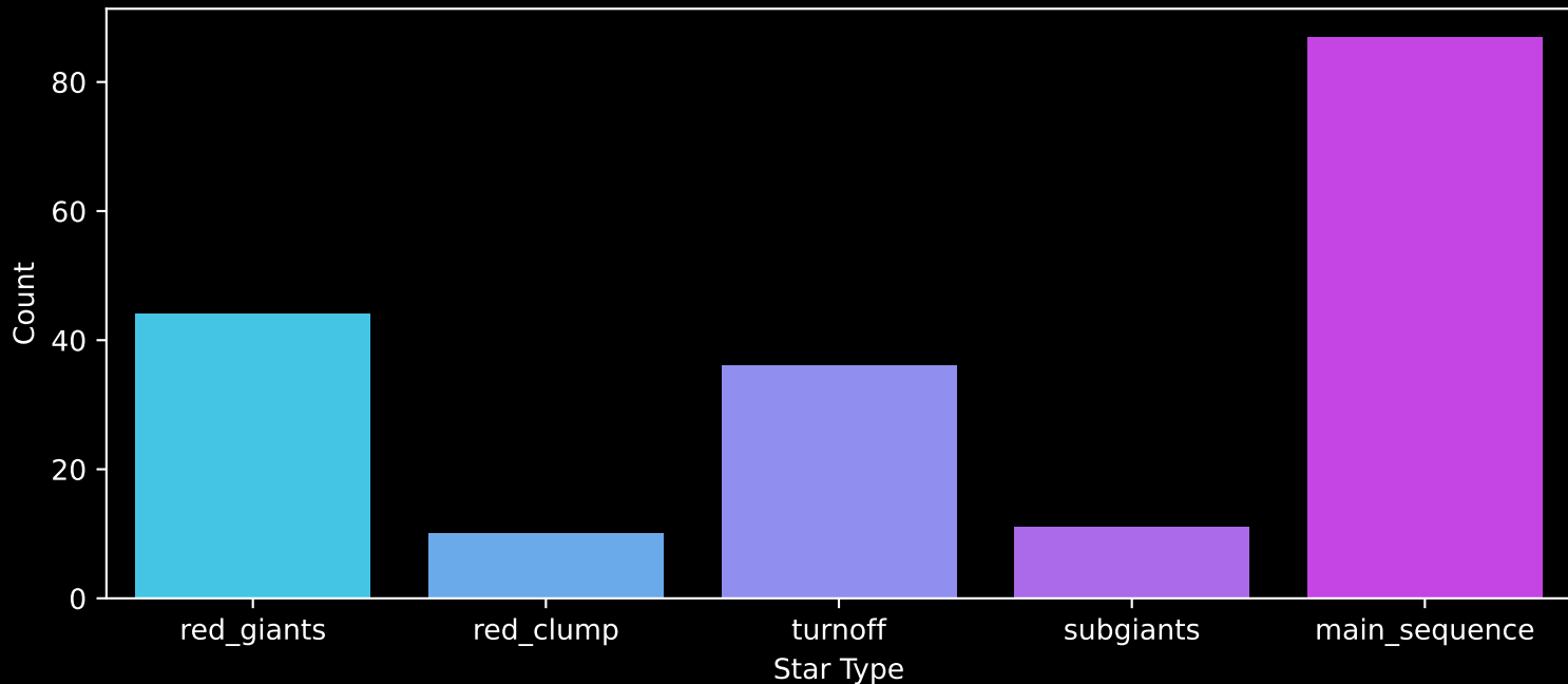
APOGEE DR17 Field: [172+32_MGA] Count plot of Star Type
