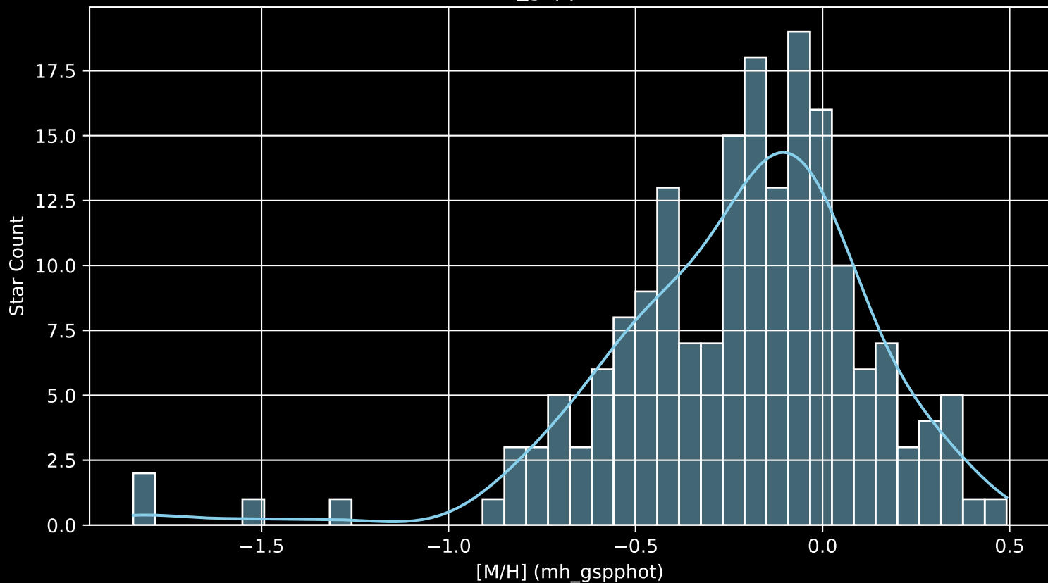
APOGEE DR17 Field: [172+32_MGA [M/H] (mh_gspphot) (n= 187)
