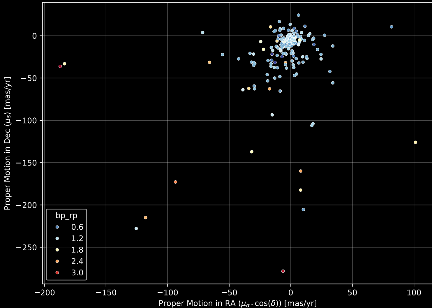
APOGEE DR17 Field: [172+32_MGA] Proper Motion Diagram (n= 188)
