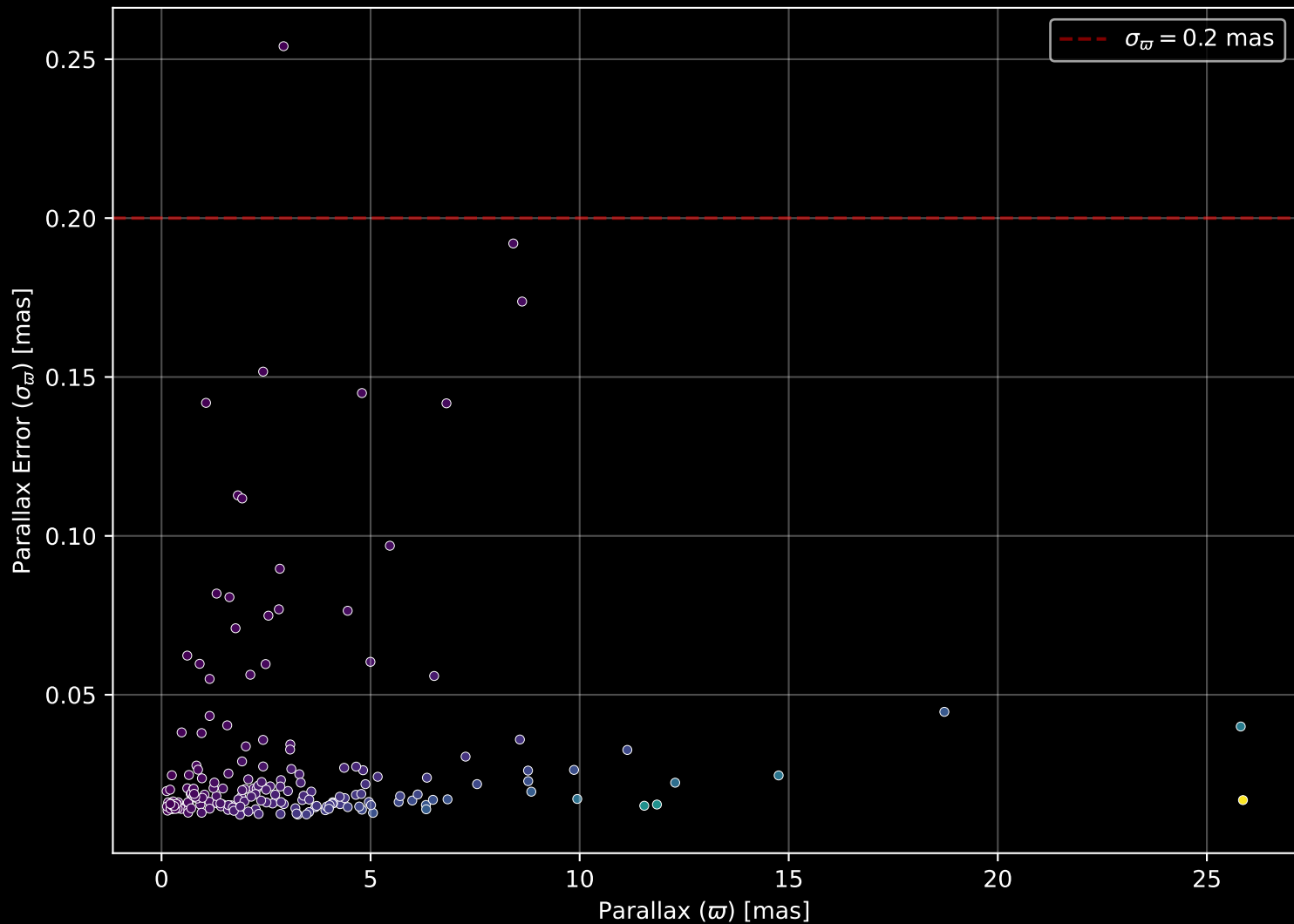
APOGEE DR17 Field: [172+32_MGA] Parallax Quality (n= 188)
