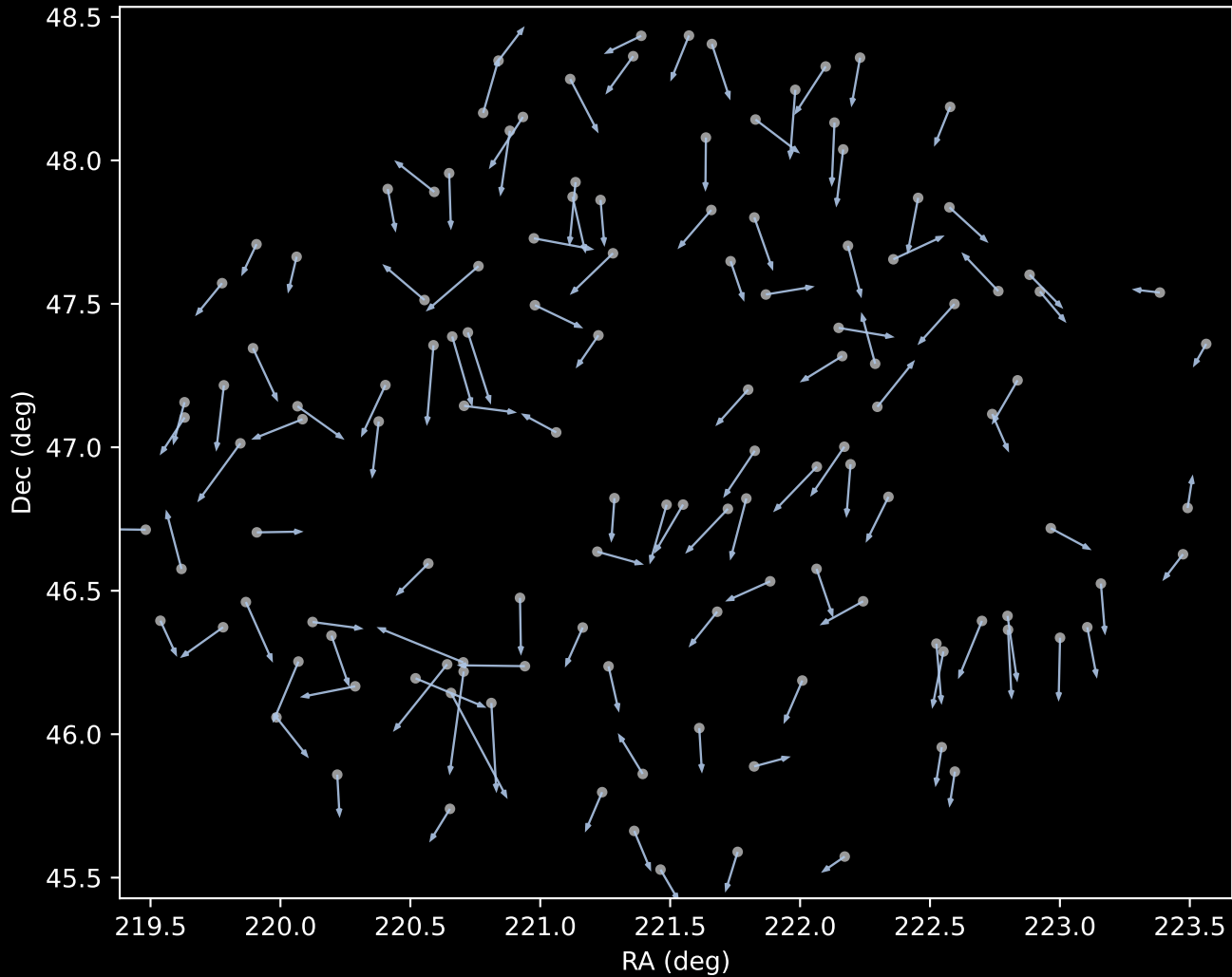
APOGEE DR17 Cluster 1 Proper Motion Vectors (n=128)
