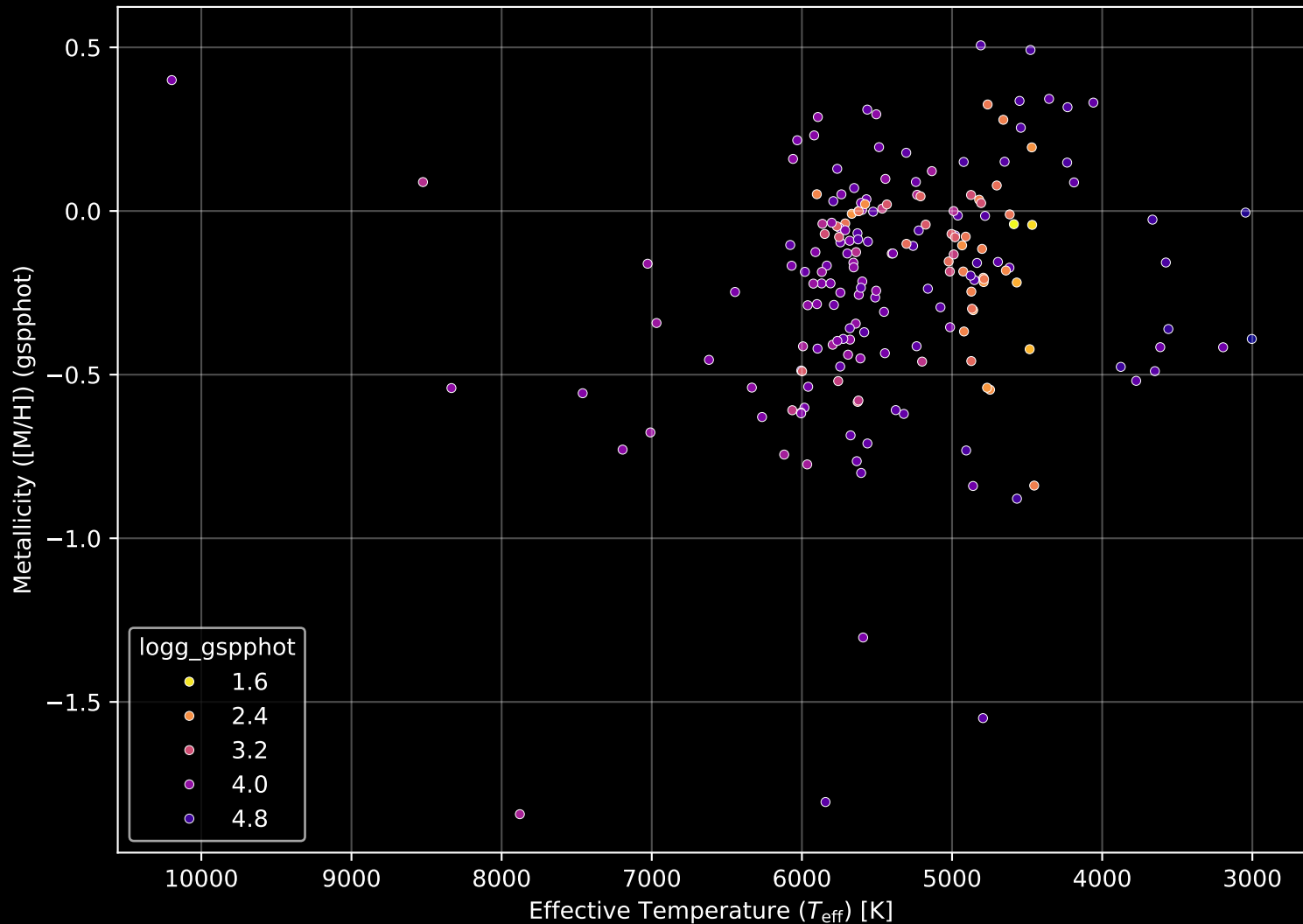
APOGEE DR17 Field: [172+32_MGA] Stellar Population Parameters (n= 188)
