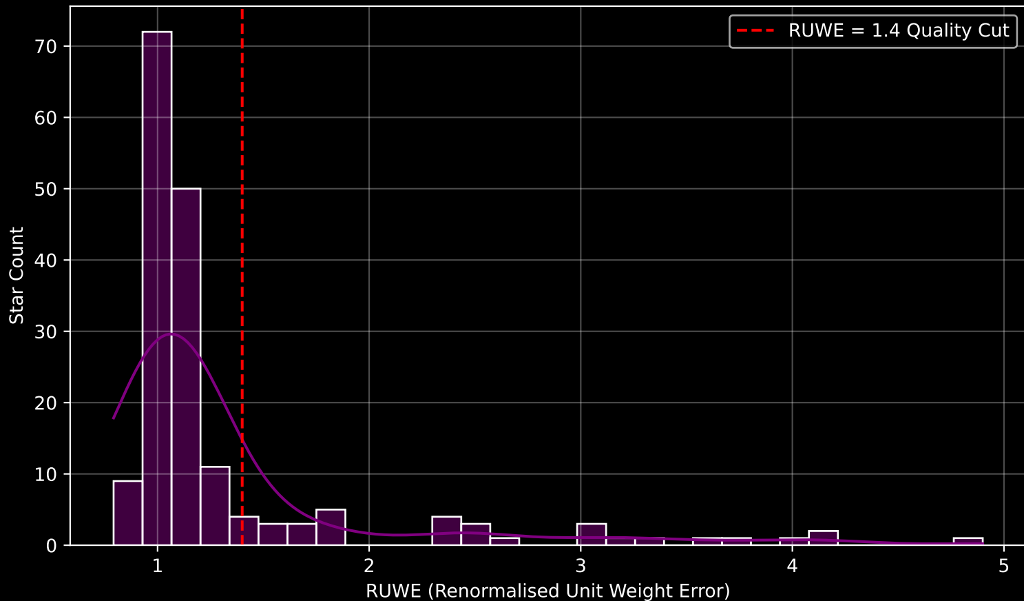
GAPOGEE DR17 Field [172+32_MGA] RUWE Distribution (n= 176)
